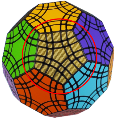
5-fold symmetry Turns 72^\circ \cdot n degrees
