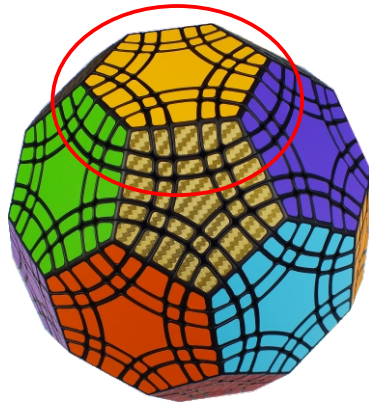
3-fold symmetry Turns 120^\circ \cdot n degrees
